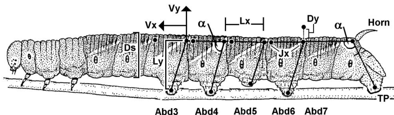
Figure 1. Marker points and parameters used to characterize the kinematics of Manduca crawling. Fluorescent beads were placed on the posterior upper insertion (UI) points of the dorsal exterior oblique muscle (DEO) on abdominal segments Abd3 through Abd6 and on the dorsal cuticle at the horn attachment in the most posterior segment. These markers were used to measure the length of the segments ( L_x ), their vertical ( V_y ), and horizontal ( V_x ), velocities, and vertical displacement ( D_y ). Markers were also applied to the anterior upper origin (UO) of DEO to measure the intrasegmental distance ( J_x ). Beads applied to the lateral distal margin of the prolegs (including the terminal prolegs, TP) were used to measure proleg movements including retraction (changes in L_y ) and swing angle ( \alpha ). The animals were illuminated with a high-intensity longwave UV lamp and their movements recorded simultaneously from two angles, using a pair of digital video cameras. Video data from each camera captured as 760 pixels \times 480 pixels at a frame rate of 29.97/s were synchronized using flashes produced from an LED and stored in uncompressed format for analysis. Segment diameter ( D_s ) was measured directly from side-view high-resolution images (3 megapixels) of freely moving caterpillars.
